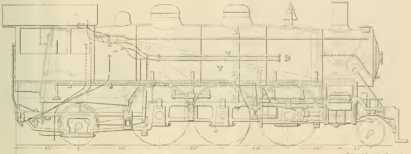
DETAILS OF ILLINOIS CENTRAL PRAIRIE TYPE
